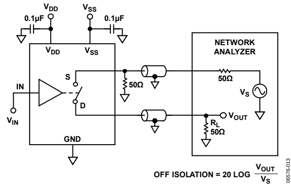
Figure 23. Off Isolation
